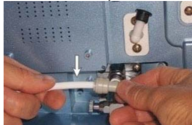
1/4" White hose to Tap Water Inlet Port
