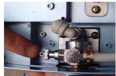
Gray Hose To Acidic Water Outlet Port
